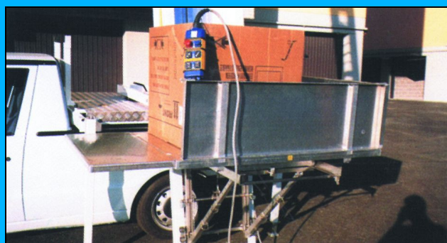
The loading platform may be rotated to fit into the windows or balcony size. A platform extension makes loading and unloading easier.
